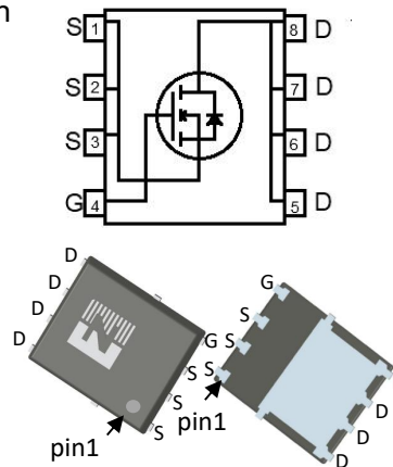
DFN5*6
